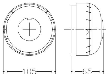
Smoke/ Heat Detector Dimensions
