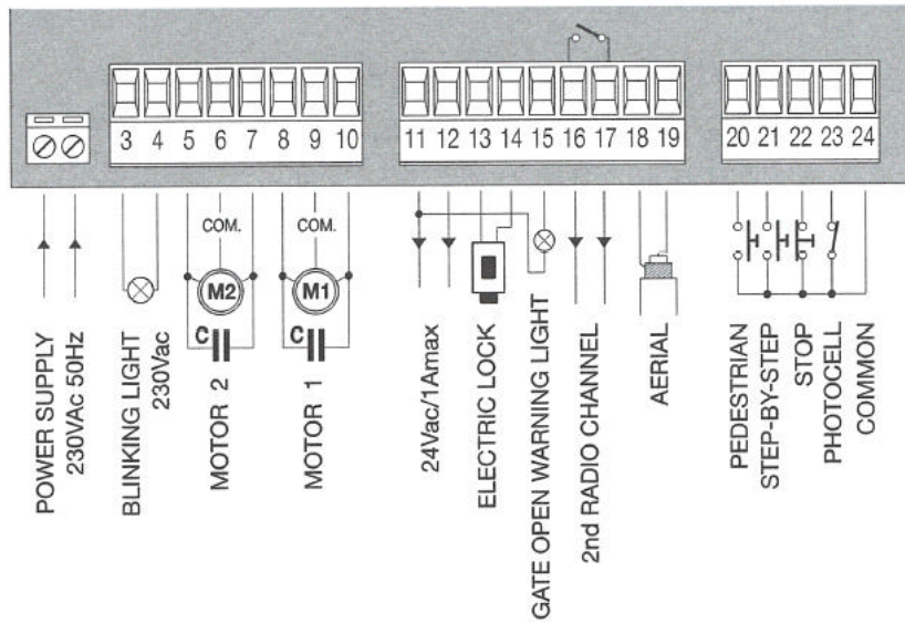
Brain Control Panel for swinging or sliding gates (for use with keypad / intercom applications)
